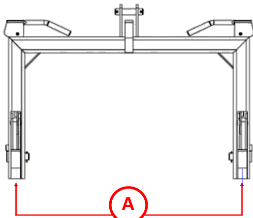
3-Point Tools 200-606
