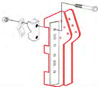
Clamping View for 2-1/4" Diamond Bar
