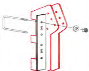
Clamping View for Flat Bar
